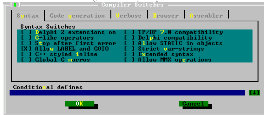
Figure 6.23: The syntax options tab
